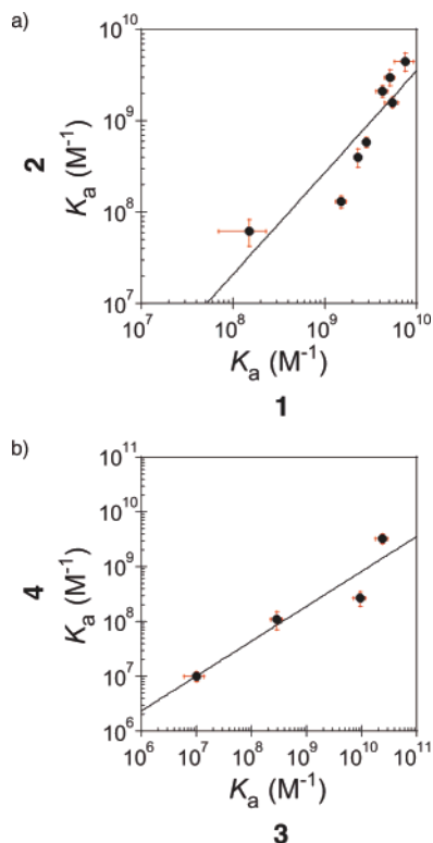
Figure 7. (a) Correlation of K_a values for polyamide 1 (fluorescein labeled) and polyamide 2 (Cy3 labeled). (b) Correlation of K_a values for polyamide 3 (unlabeled) and polyamide 4 (Cy3 labeled).
