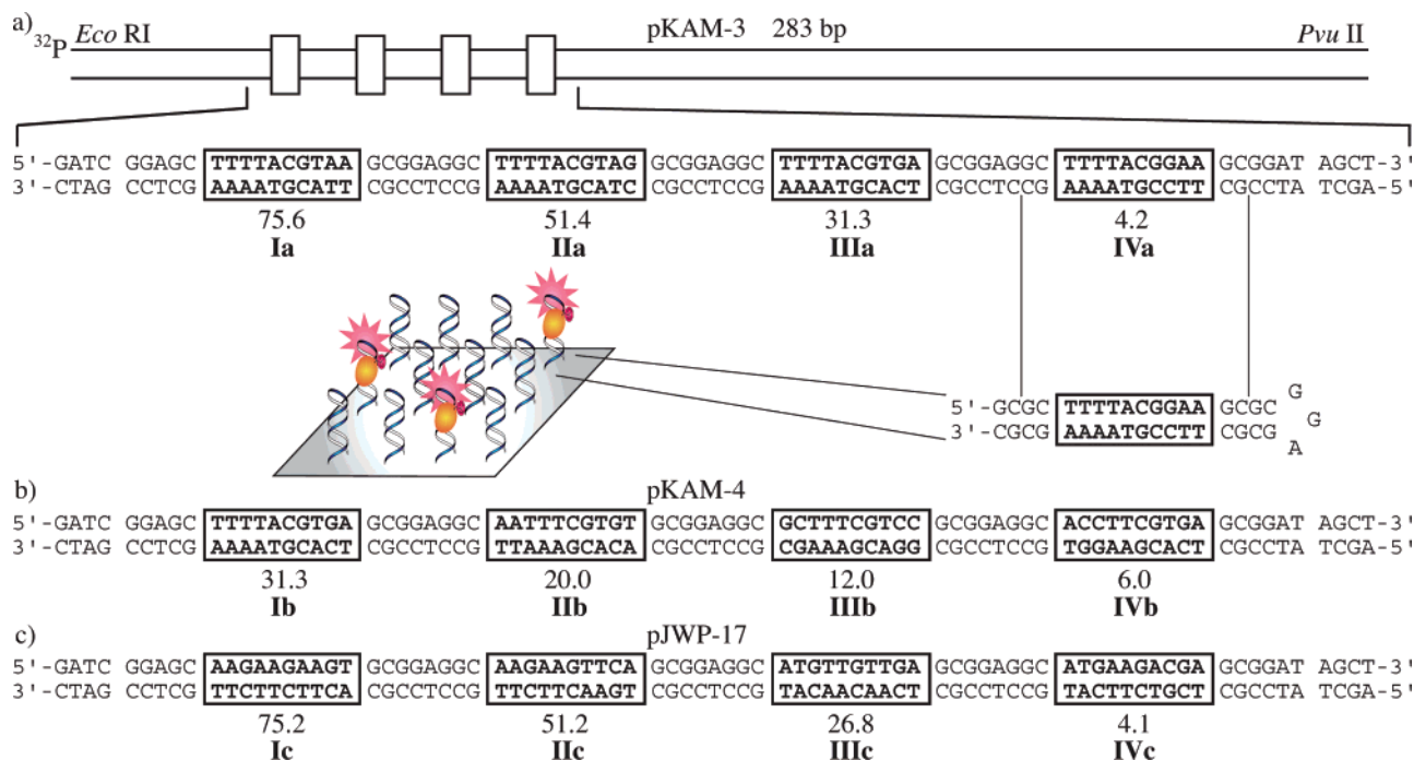
Figure 3. Insert sequences utilized for plasmids, with binding sites boxed, labeled with their corresponding CSI array intensity, and numbered. (a) pKAM3 is shown, in addition to a microarray schematic demonstrating the relationship between the plasmid and a selected microarray sequence. (b) pKAM4. (c) pJWP17.
