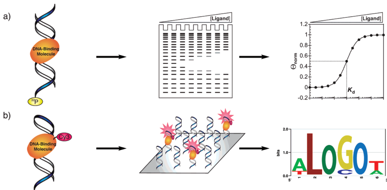
Figure 1. (a) Quantitative DNase I footprinting gives rise to a defined equilibrium association constant at a specified binding site for a given DNA binding molecule. (b) The CSI microarray platform gives rise to relative binding preferences of an entire sequence space for the same molecule with a sequence logo as a standard summary output.
