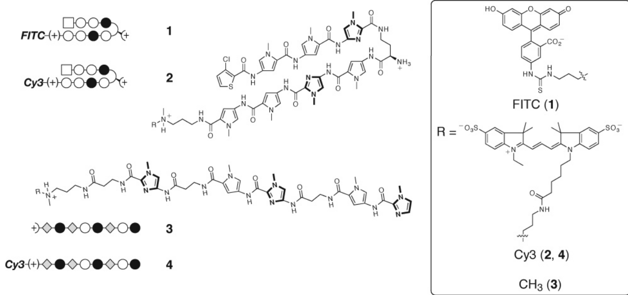
Figure 2. Hairpin polyamides 1 and 2 targeted to the hypoxia response element (HRE), 5'-TACGTG-3'. Linear \beta -linked polyamides 3 and 4 targeted to GAA repeats in Friedrich's Ataxia.
