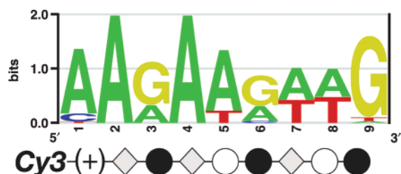
Figure 9. Sequence logo for polyamide 4.
