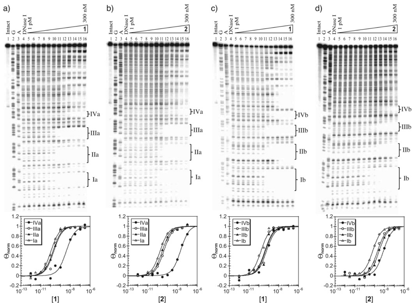
Figure 4. DNase I footprinting gels and corresponding isotherms of polyamides 1 and 2 on pKAM3 and pKAM4. (a) Polyamide 1 on pKAM3. (b) Polyamide 2 on pKAM3. (c) Polyamide 1 on pKAM4. (d) Polyamide 2 on pKAM4.
